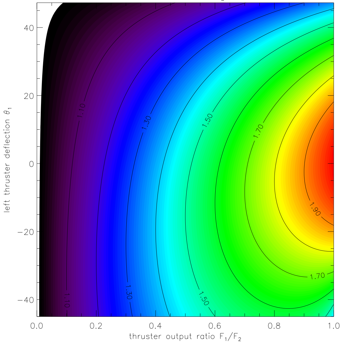
total thrust: TIE Fighter
